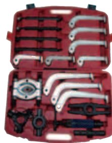
800-CSSC1710 綜合型油壓拔卸器組 MULTI-HYDRAULIC GEAR PULLER KIT
