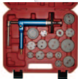
705-CSSC1050 氣動煞車分泵調整組 AIR POWERED BRAKE CALIPER WIND BACK TOOL SET
