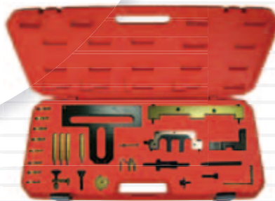
601-CSSC8092 BMW正時工具 ENGINE TIMING TOOL SET FOR PROFESSIONAL ENGINE REPAIR BMW N42/N46/N46T
